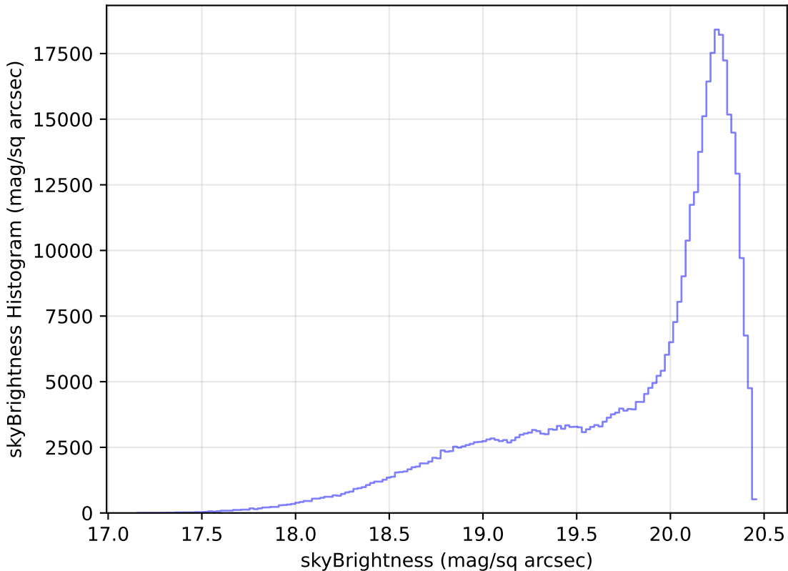
baseline_v2.1_10yrs WFD i band: skyBrightness Histogram
