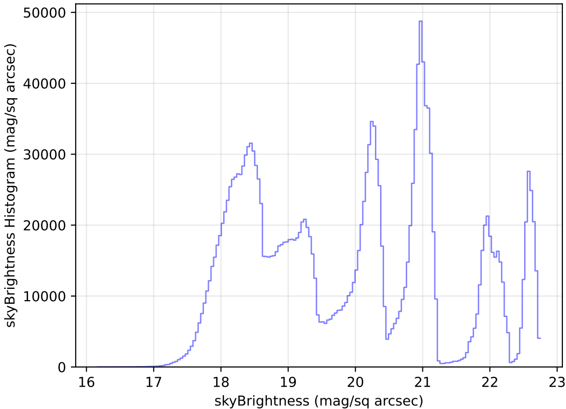
baseline_v2.1_10yrs WFD all bands: skyBrightness Histogram
