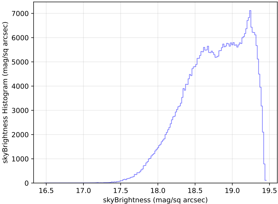
baseline_v2.1_10yrs All sky z band: skyBrightness Histogram
