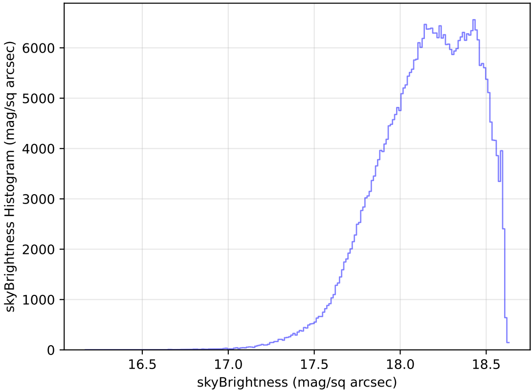
baseline_v2.1_10yrs All sky y band: skyBrightness Histogram
