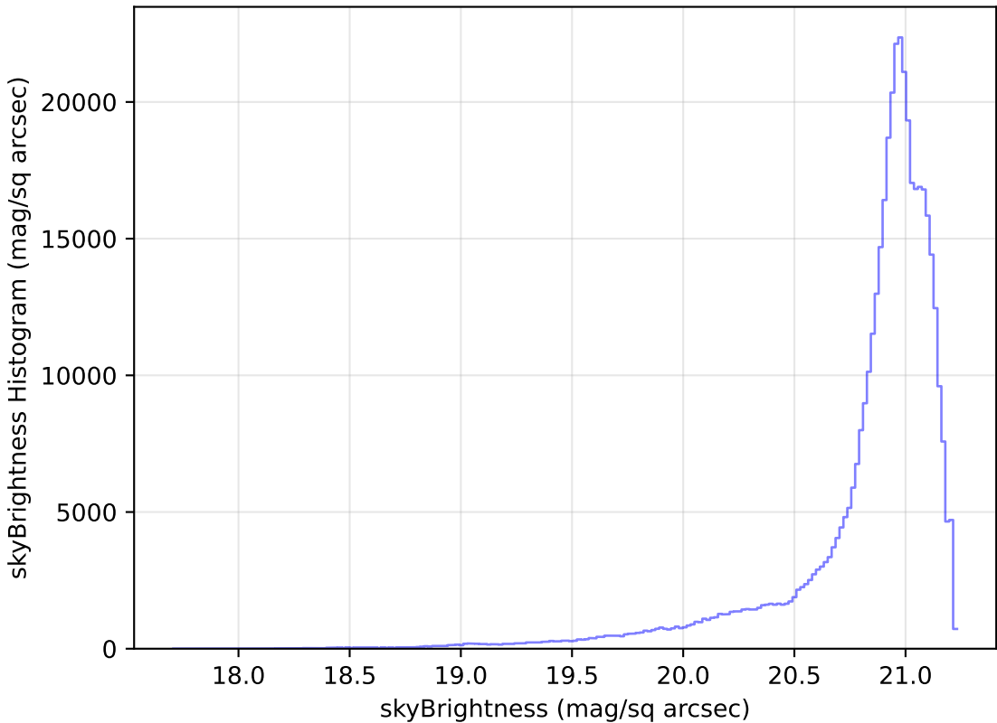
baseline_v2.1_10yrs All sky r band: skyBrightness Histogram
