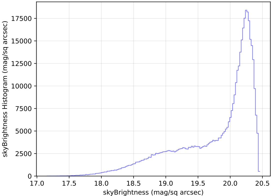
baseline_v2.1_10yrs All sky i band: skyBrightness Histogram
