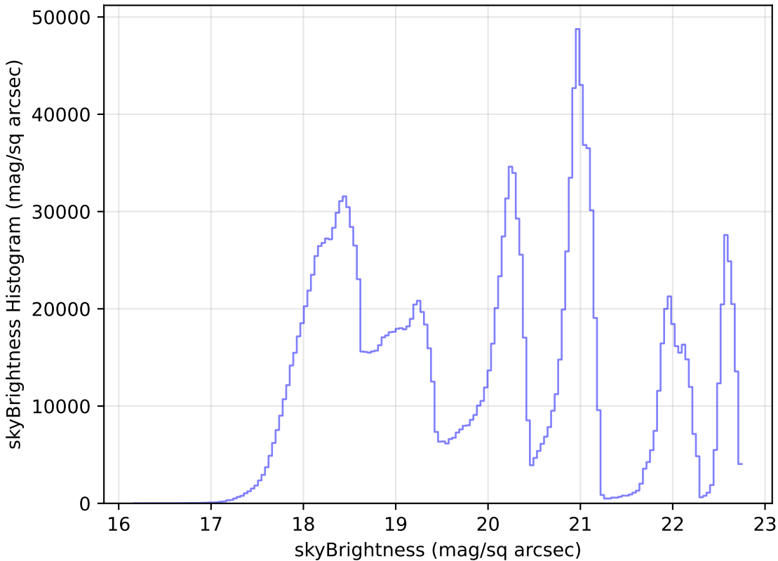
baseline_v2.1_10yrs All sky all bands: skyBrightness Histogram
