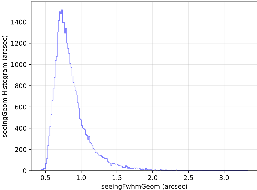
baseline_v2.1_10yrs Yr 1 z band: seeingGeom Histogram
