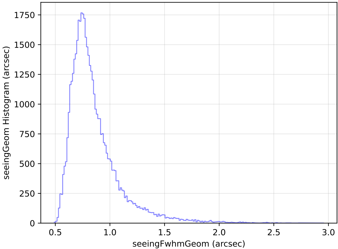
baseline_v2.1_10yrs Yr 1 y band: seeingGeom Histogram
