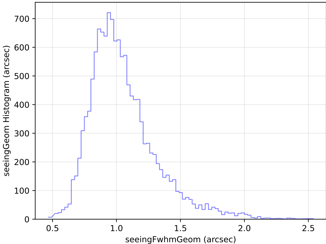
baseline_v2.1_10yrs Yr 1 u band: seeingGeom Histogram
