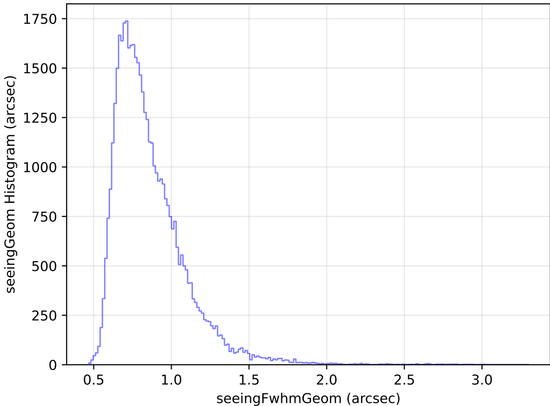
baseline_v2.1_10yrs Yr 1 r band: seeingGeom Histogram
