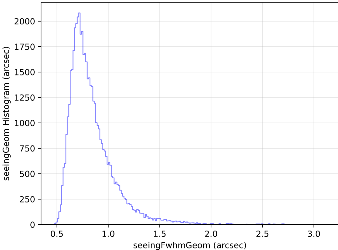
baseline_v2.1_10yrs Yr 1 i band: seeingGeom Histogram
