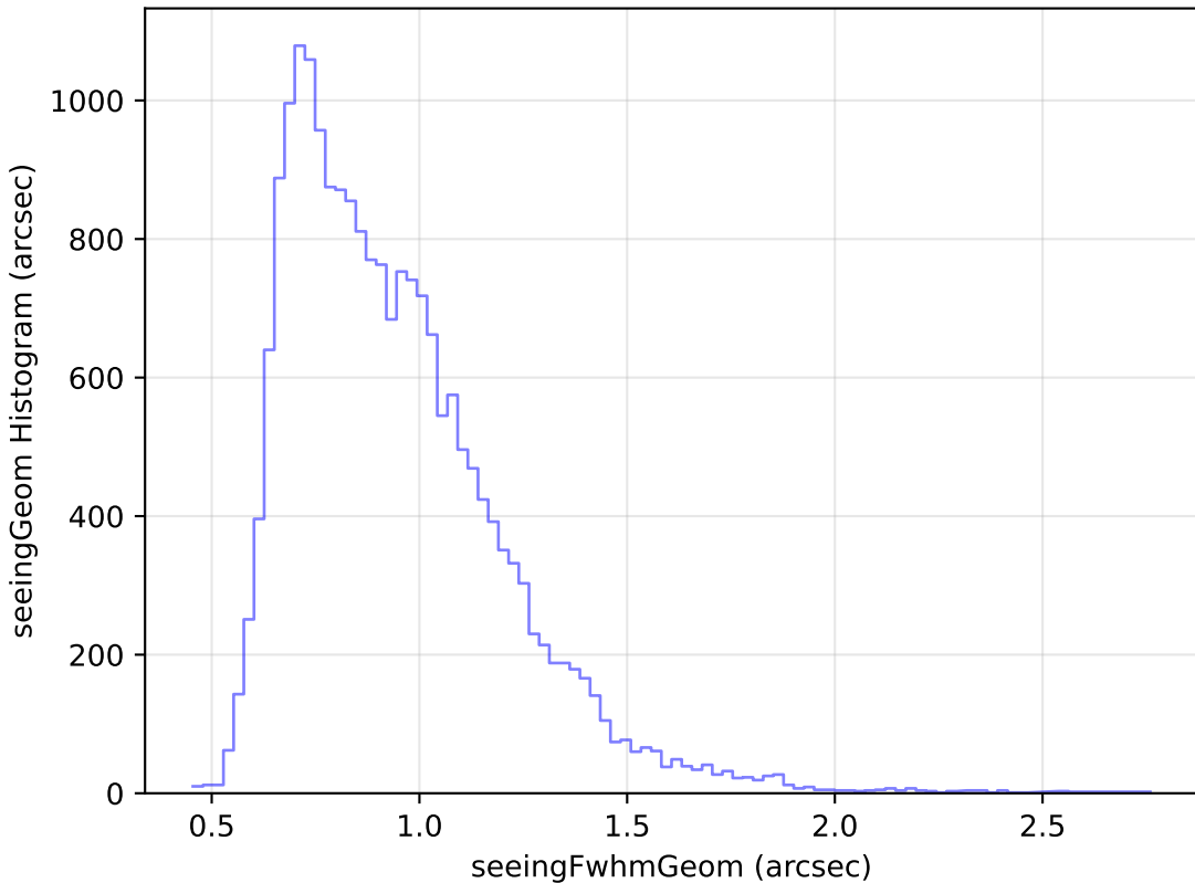
baseline_v2.1_10yrs Yr 1 g band: seeingGeom Histogram
