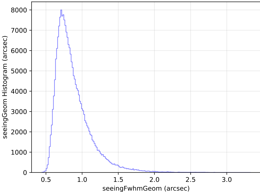
baseline_v2.1_10yrs Yr 1 all bands: seeingGeom Histogram
