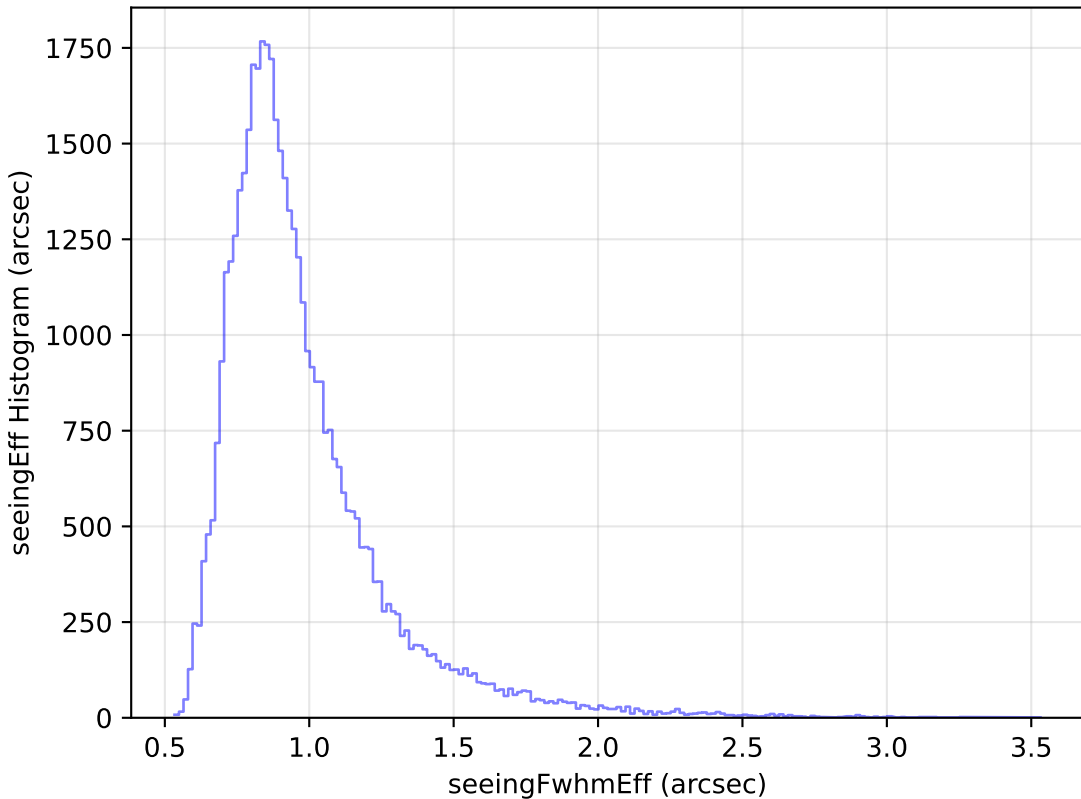
baseline_v2.1_10yrs Yr 1 y band: seeingEff Histogram
