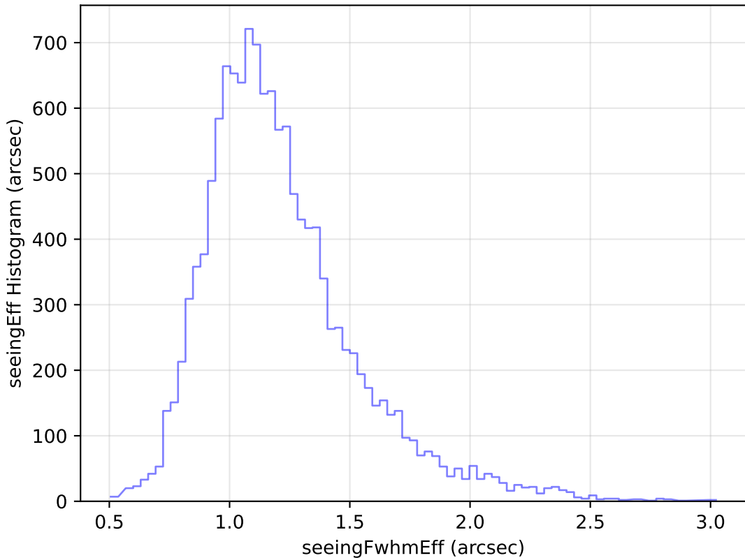
baseline_v2.1_10yrs Yr 1 u band: seeingEff Histogram
