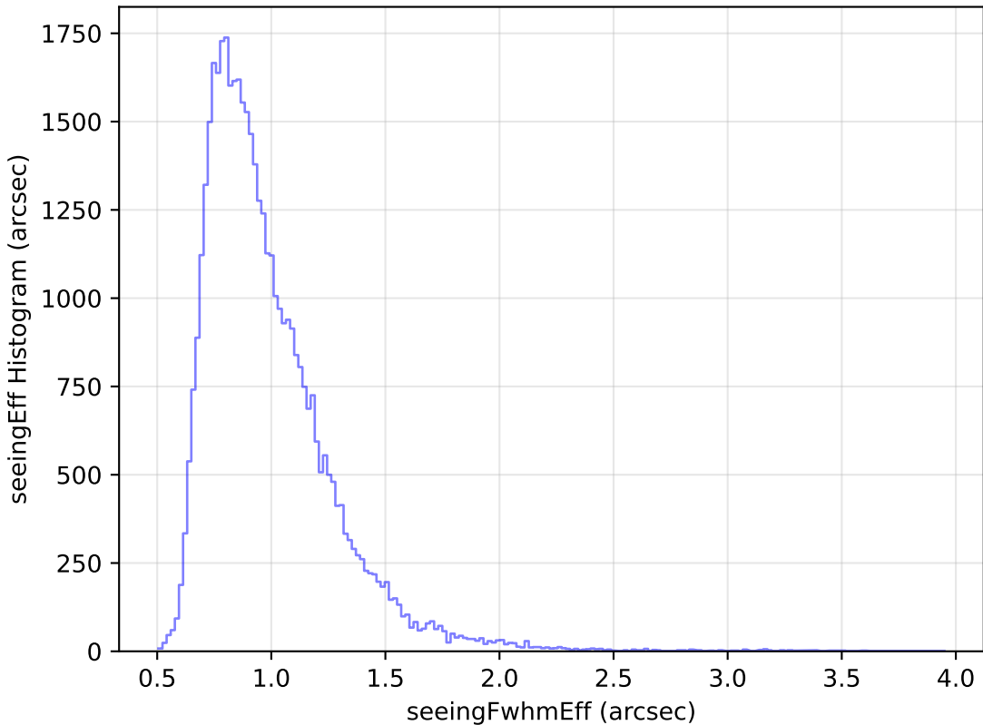
baseline_v2.1_10yrs Yr 1 r band: seeingEff Histogram
