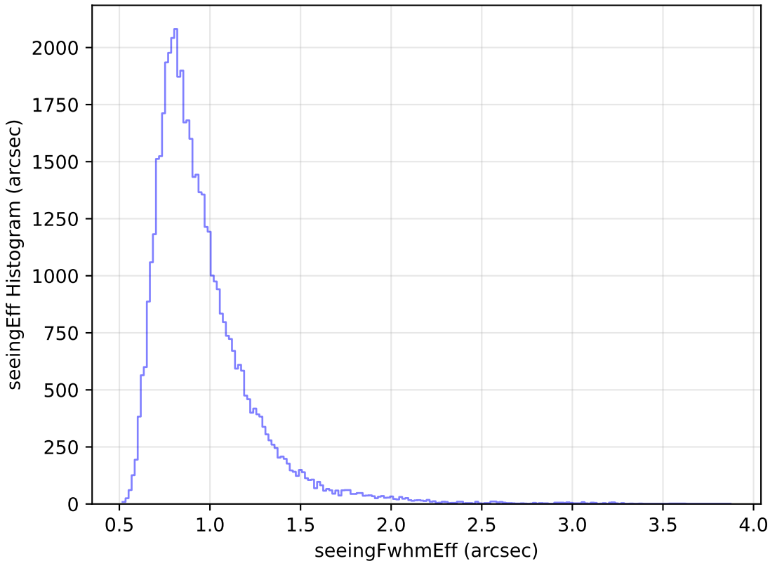
baseline_v2.1_10yrs Yr 1 i band: seeingEff Histogram
