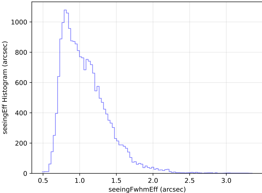
baseline_v2.1_10yrs Yr 1 g band: seeingEff Histogram
