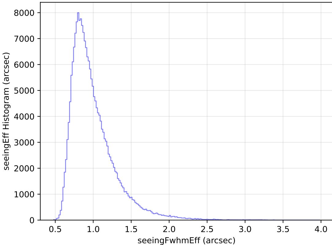
baseline_v2.1_10yrs Yr 1 all bands: seeingEff Histogram
