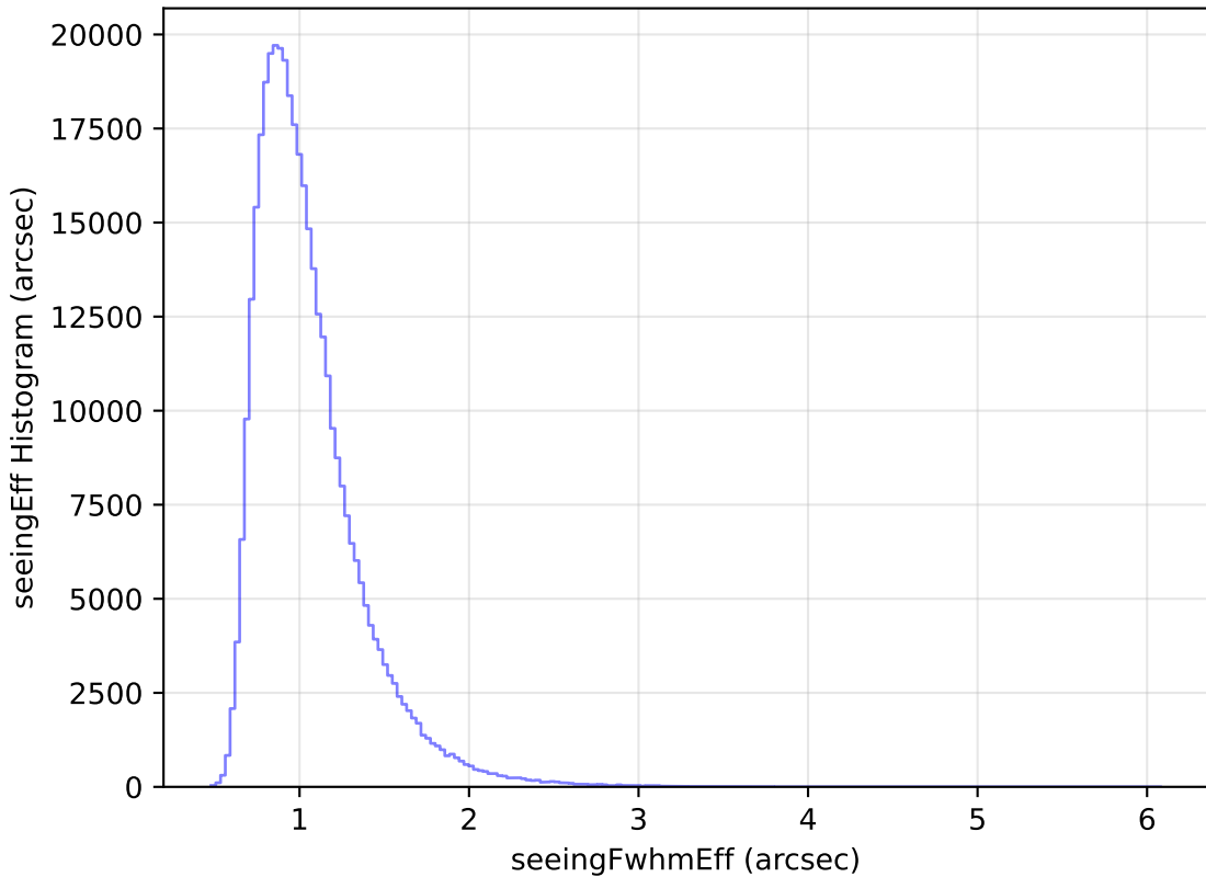
baseline_v2.1_10yrs WFD z band: seeingEff Histogram
