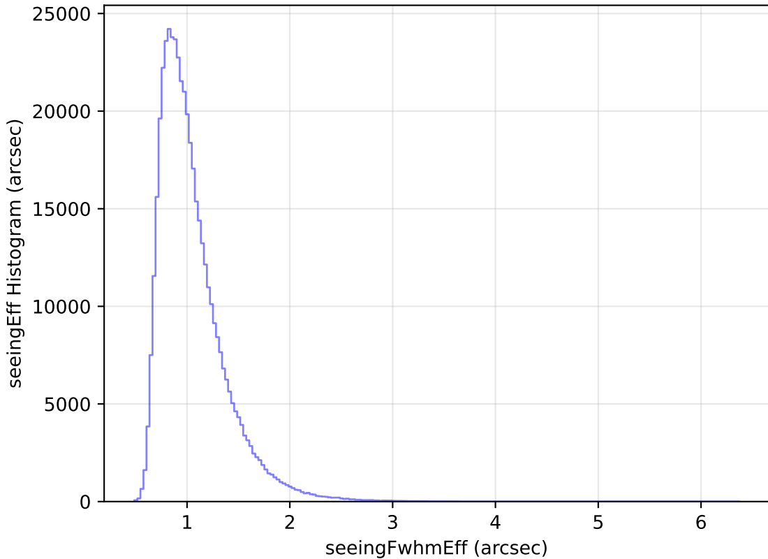
baseline_v2.1_10yrs WFD i band: seeingEff Histogram
