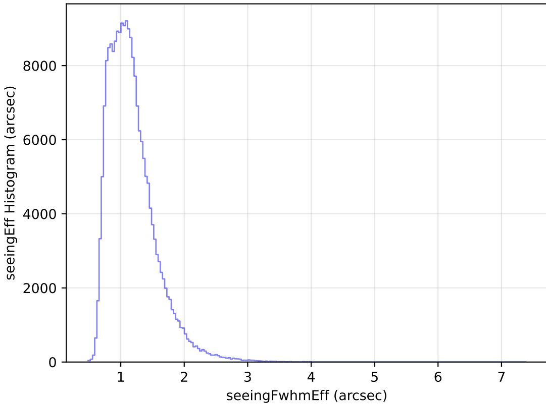
baseline_v2.1_10yrs WFD g band: seeingEff Histogram
