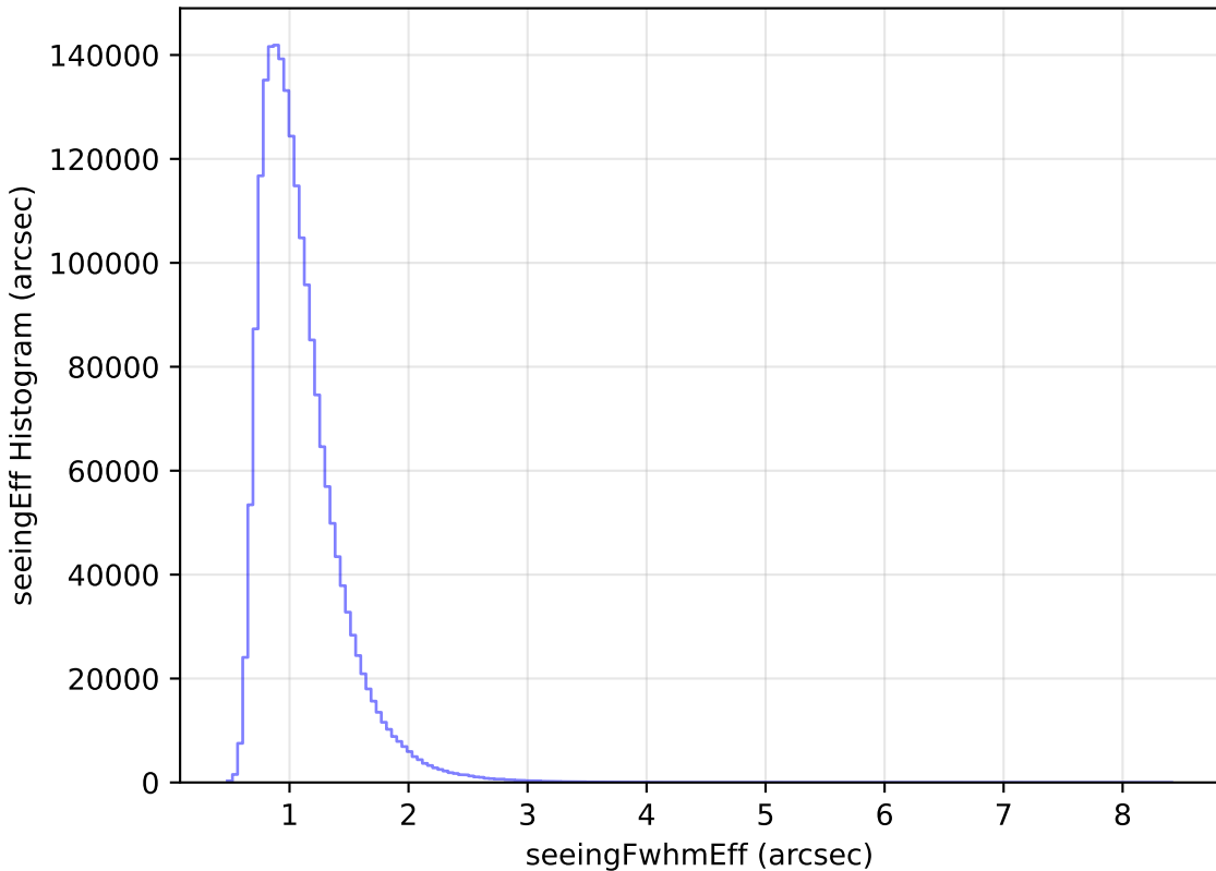
baseline_v2.1_10yrs WFD all bands: seeingEff Histogram
