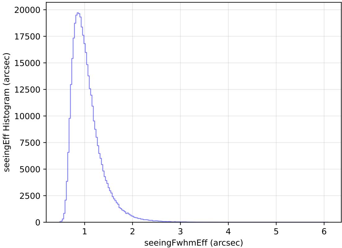
baseline_v2.1_10yrs All sky z band: seeingEff Histogram
