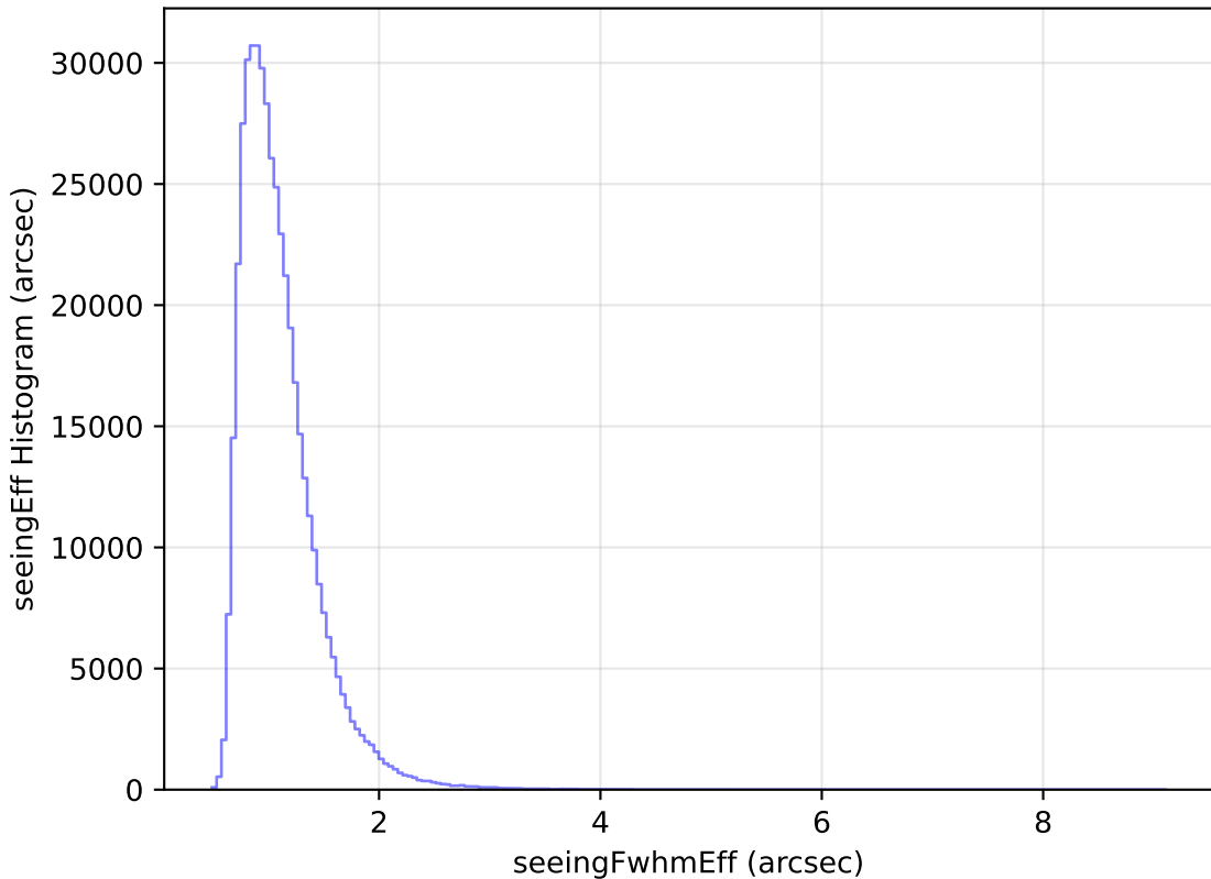
baseline_v2.1_10yrs All sky r band: seeingEff Histogram
