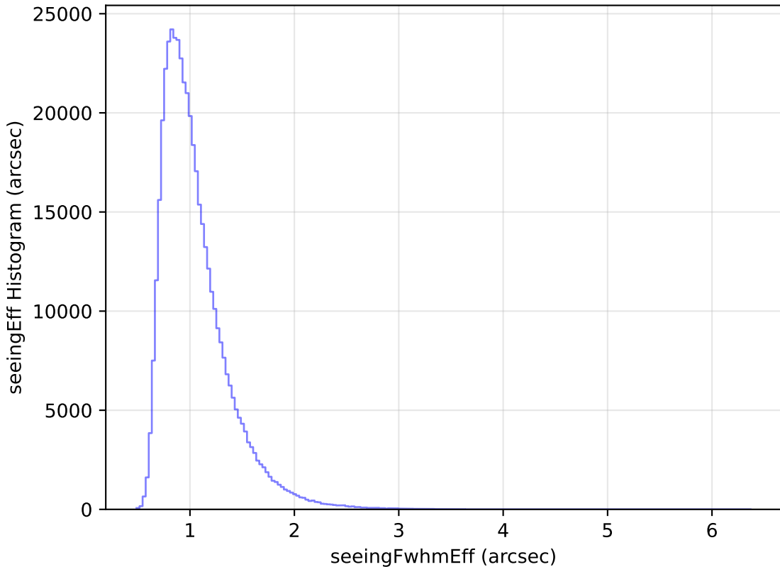
baseline_v2.1_10yrs All sky i band: seeingEff Histogram
