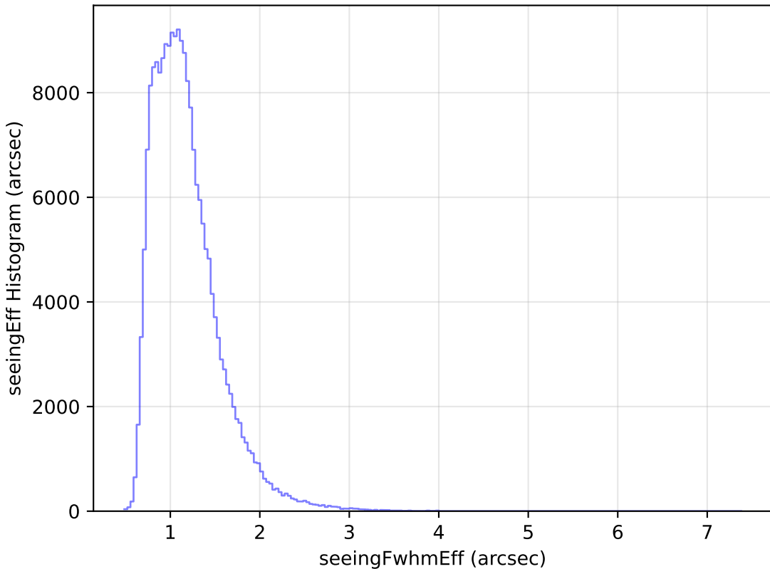
baseline_v2.1_10yrs All sky g band: seeingEff Histogram
