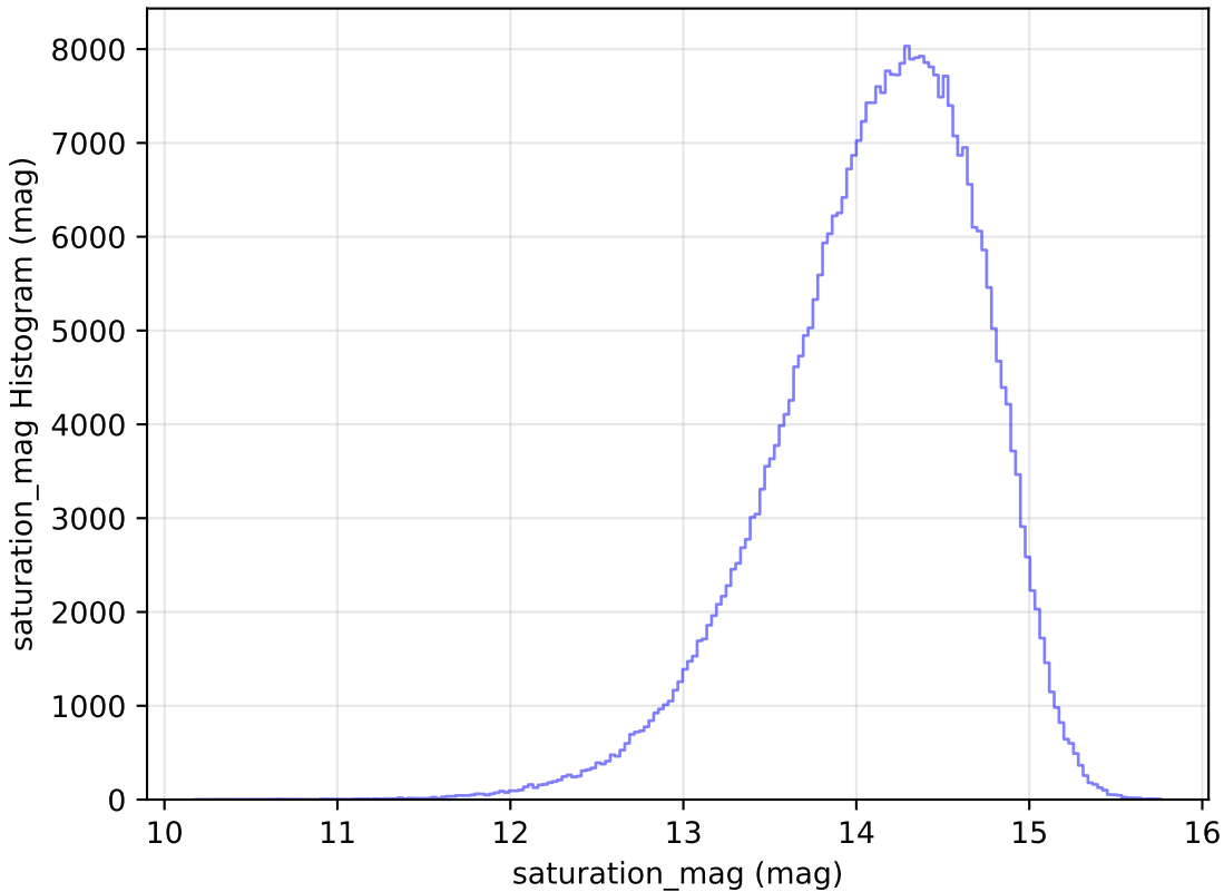
baseline_v2.1_10yrs WFD z band: saturation_mag Histogram
