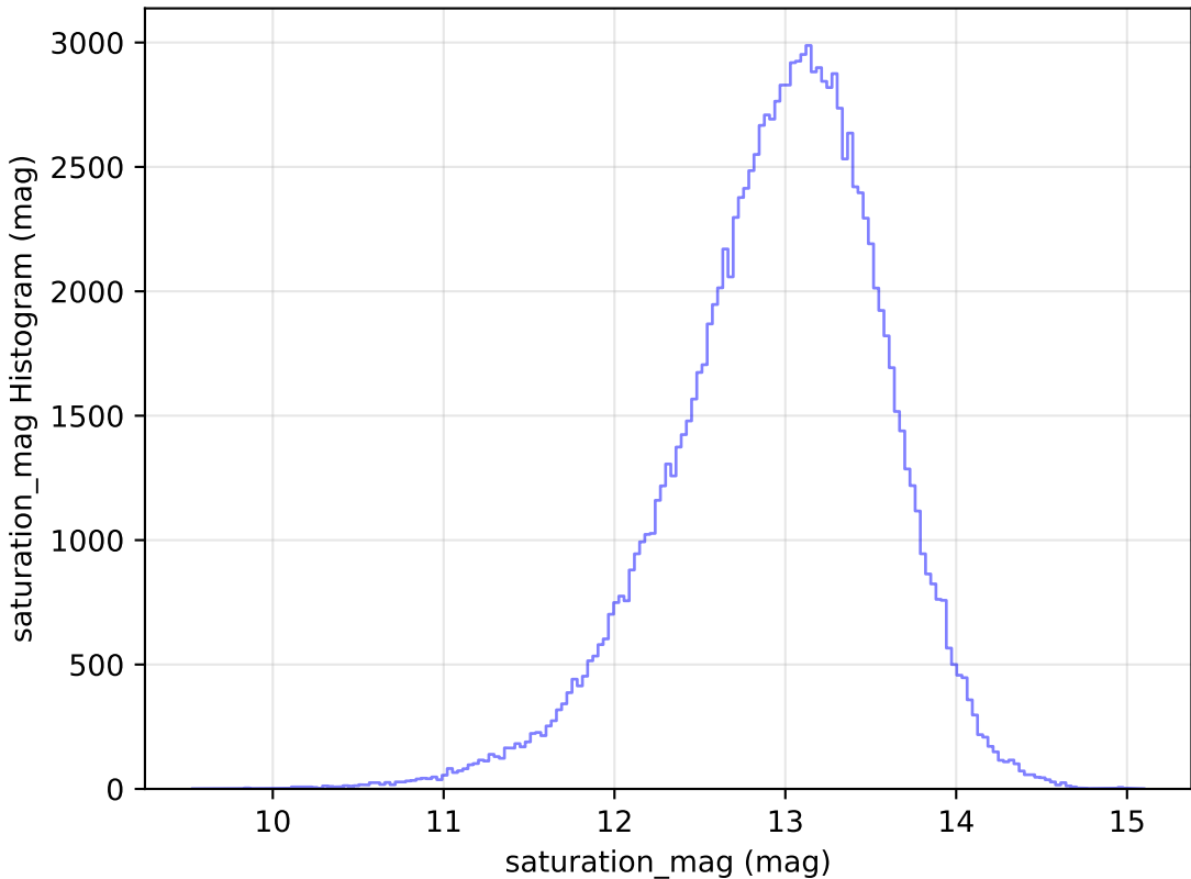
baseline_v2.1_10yrs WFD u band: saturation_mag Histogram
