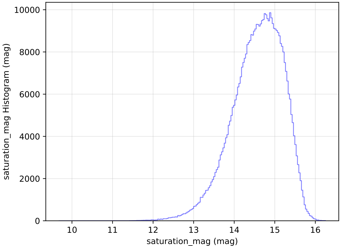
baseline_v2.1_10yrs WFD r band: saturation_mag Histogram
