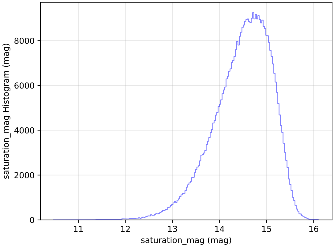
baseline_v2.1_10yrs WFD i band: saturation_mag Histogram
