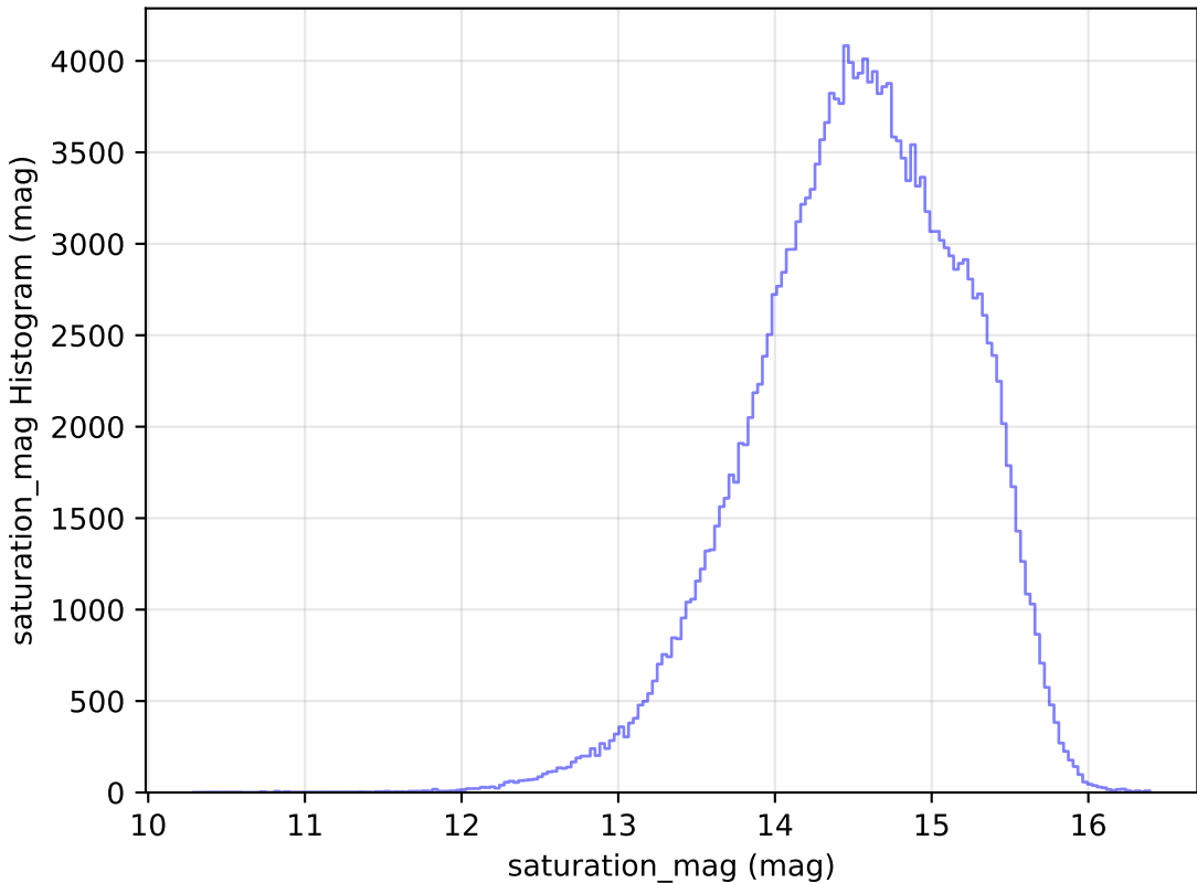
baseline_v2.1_10yrs WFD g band: saturation_mag Histogram
