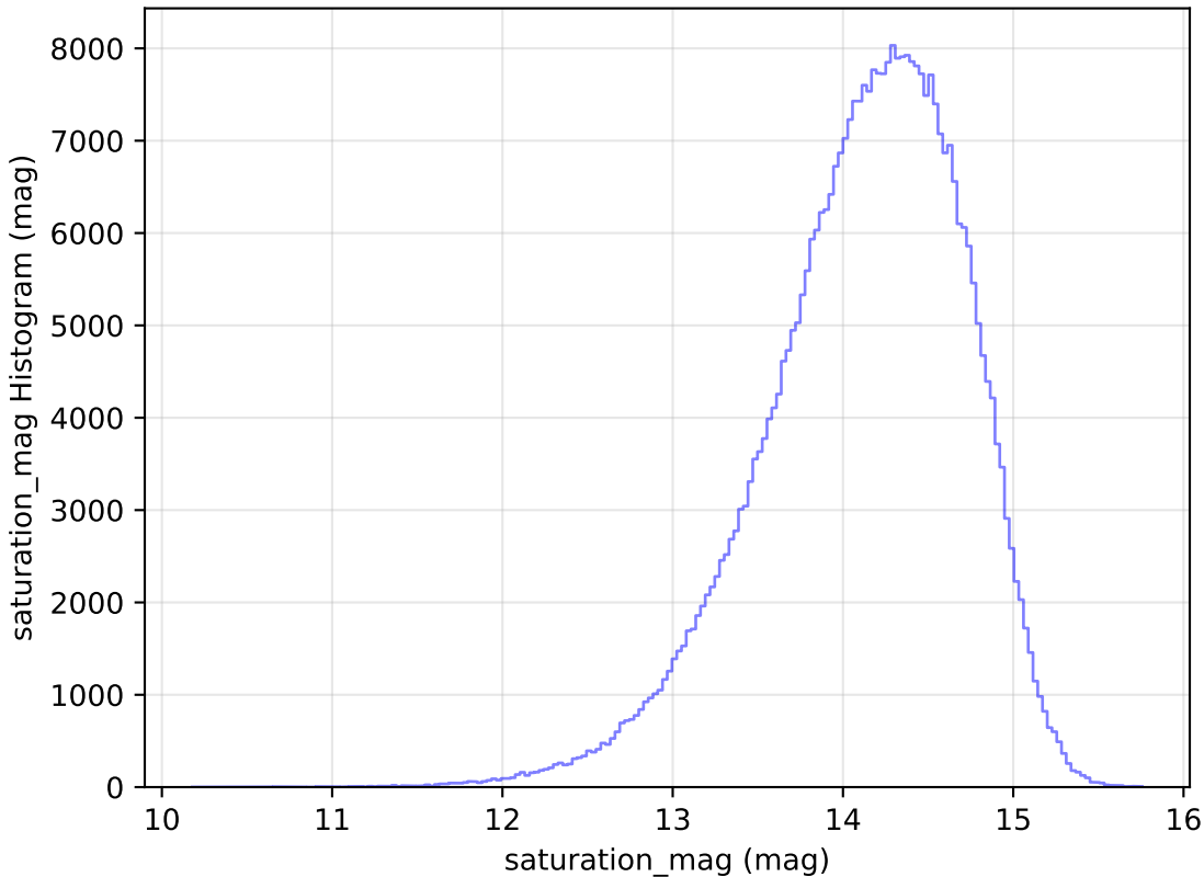
baseline_v2.1_10yrs All sky z band: saturation_mag Histogram
