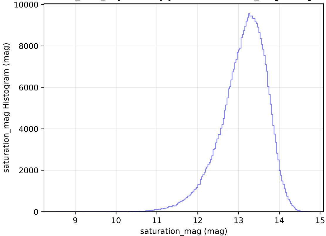
baseline_v2.1_10yrs All sky y band: saturation_mag Histogram
