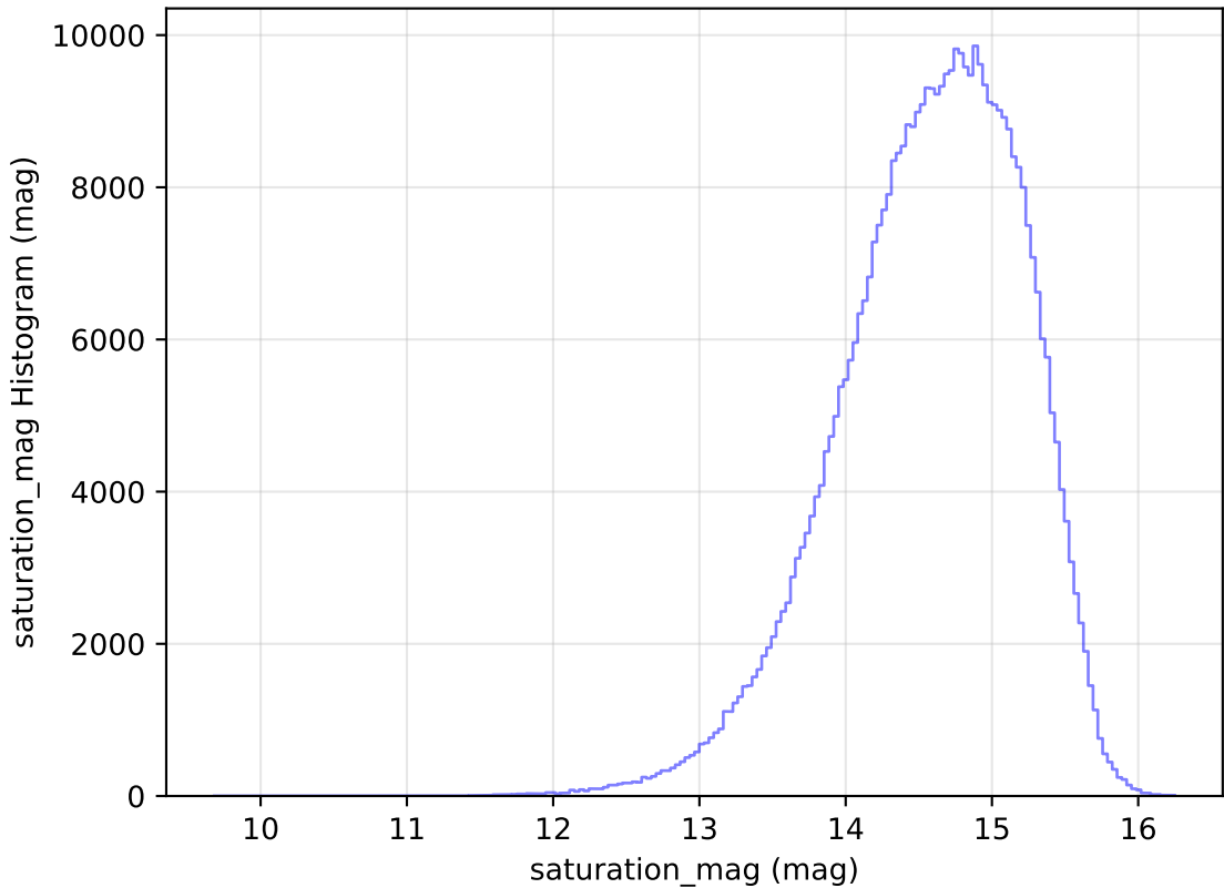
baseline_v2.1_10yrs All sky r band: saturation_mag Histogram
