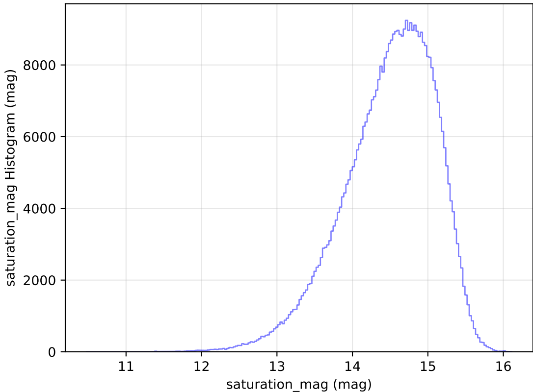
baseline_v2.1_10yrs All sky i band: saturation_mag Histogram
