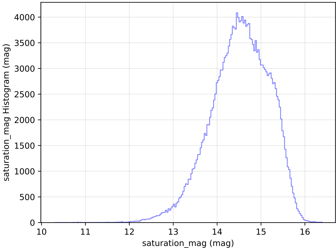
baseline_v2.1_10yrs All sky g band: saturation_mag Histogram
