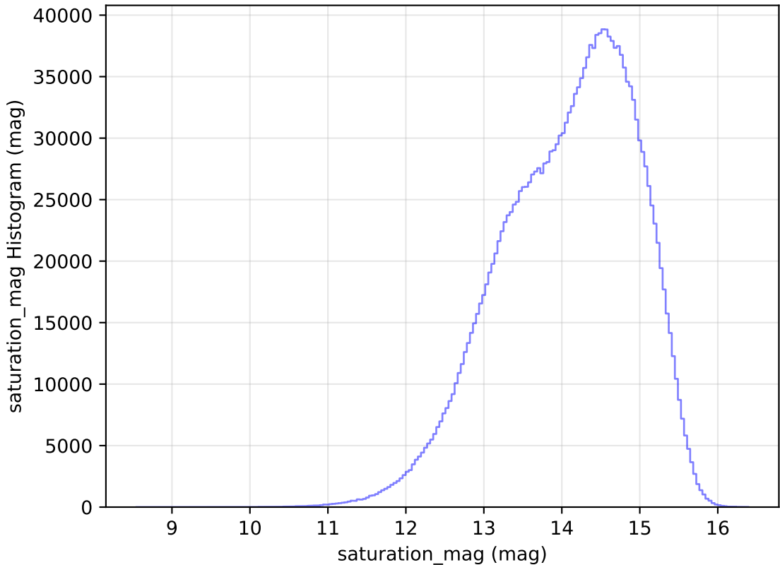
baseline_v2.1_10yrs All sky all bands: saturation_mag Histogram
