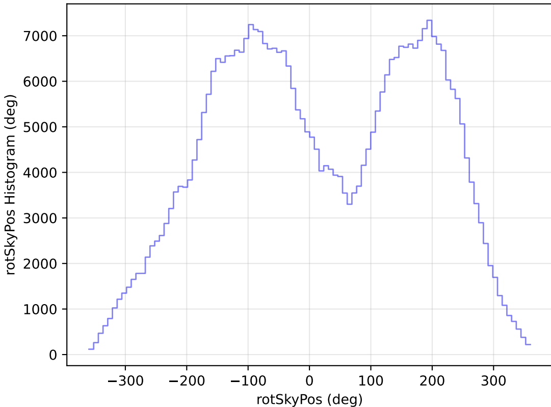
baseline_v2.1_10yrs WFD z band: rotSkyPos Histogram
