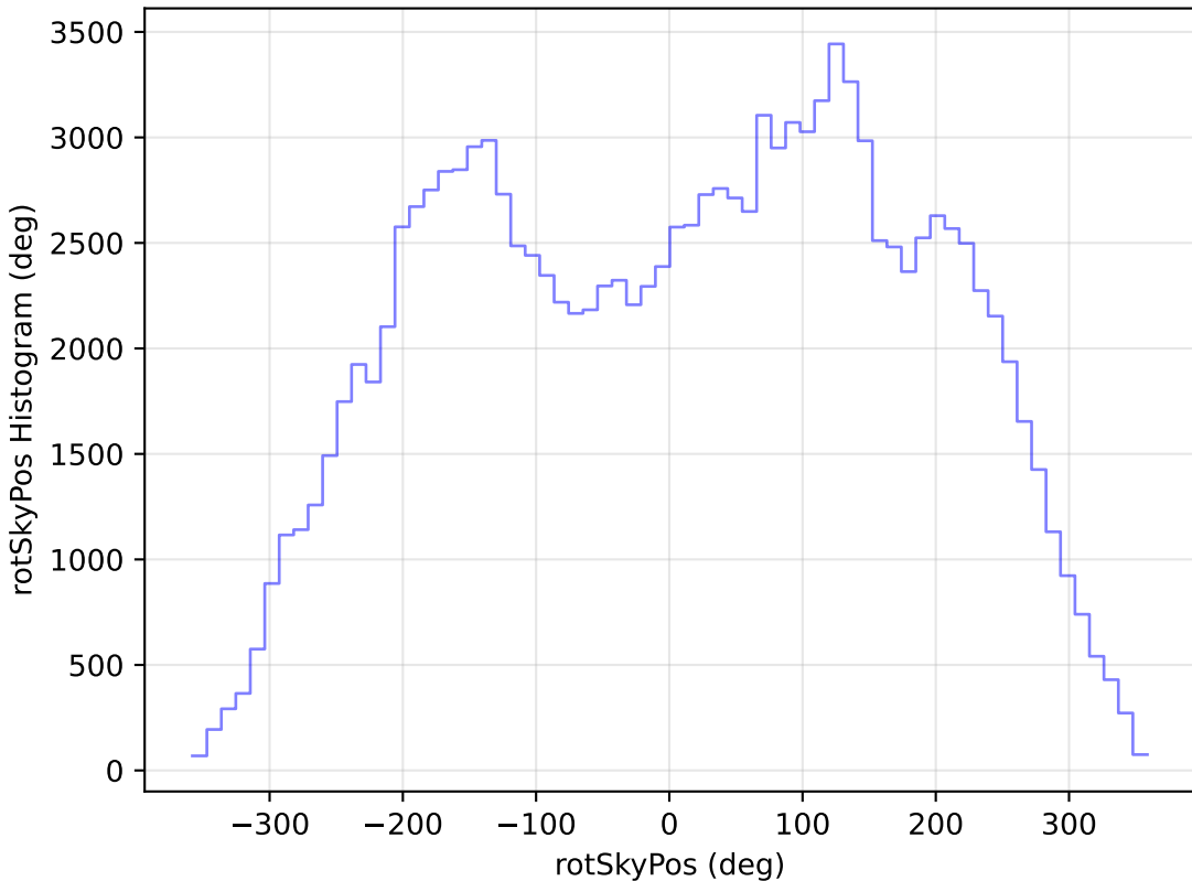
baseline_v2.1_10yrs WFD u band: rotSkyPos Histogram
