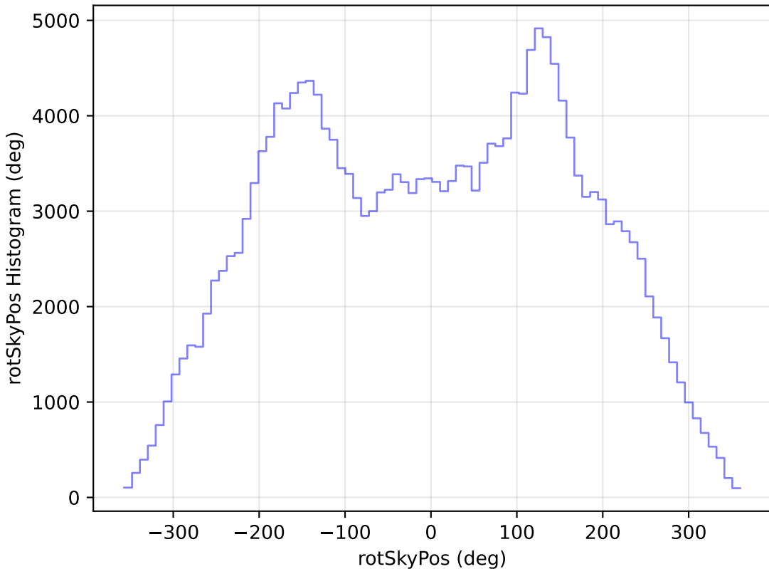
baseline_v2.1_10yrs WFD g band: rotSkyPos Histogram
