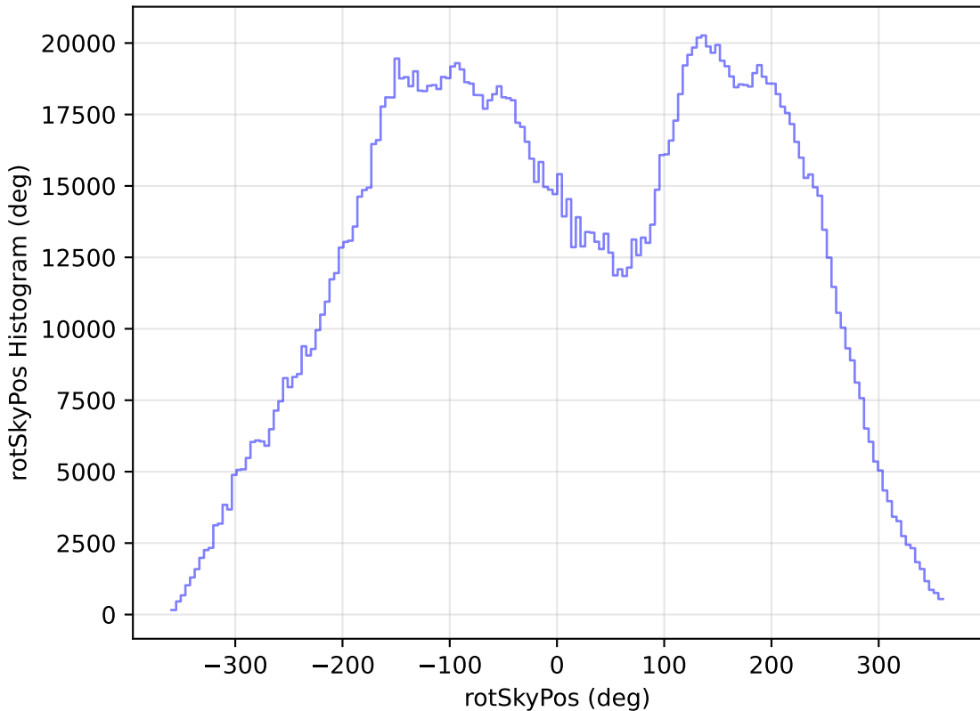
baseline_v2.1_10yrs WFD all bands: rotSkyPos Histogram
