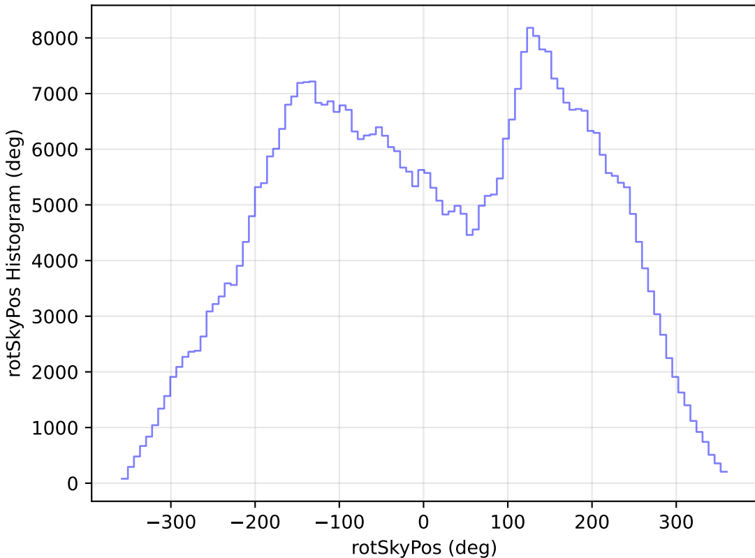
baseline_v2.1_10yrs All sky r band: rotSkyPos Histogram
