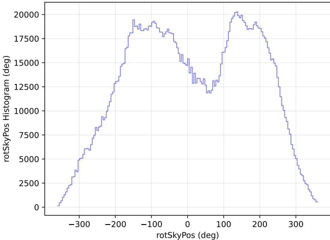
baseline_v2.1_10yrs All sky all bands: rotSkyPos Histogram
