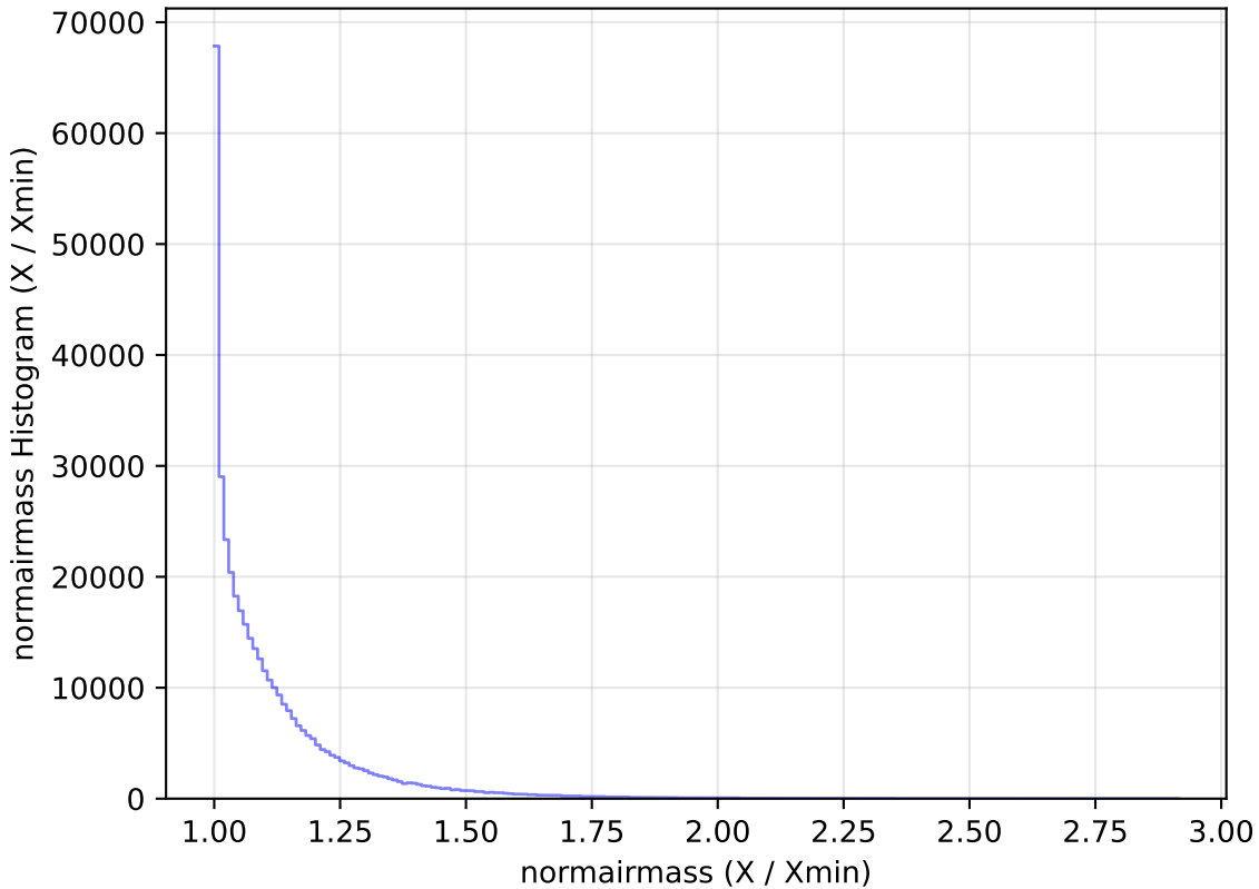
baseline_v2.1_10yrs WFD z band: normairmass Histogram
