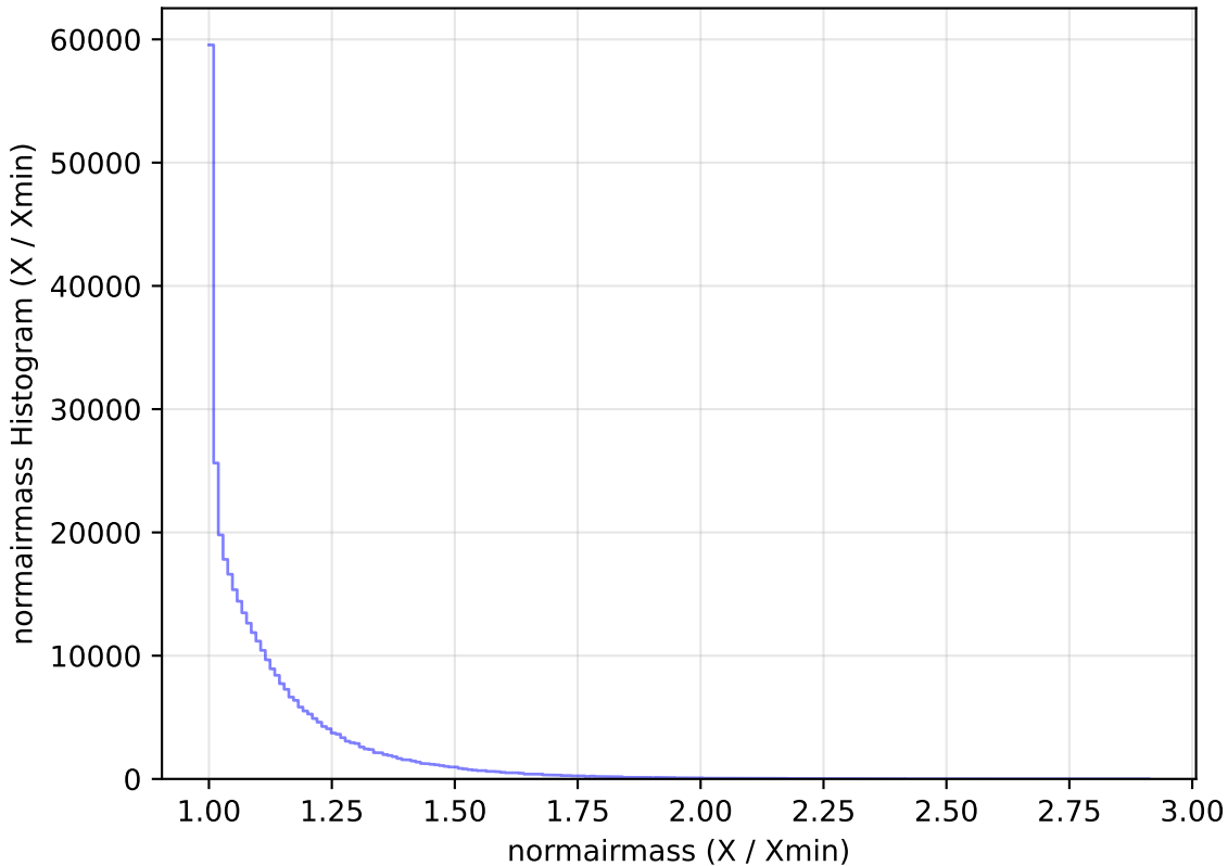
baseline_v2.1_10yrs WFD y band: normairmass Histogram
