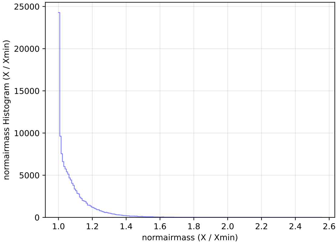
baseline_v2.1_10yrs WFD u band: normairmass Histogram
