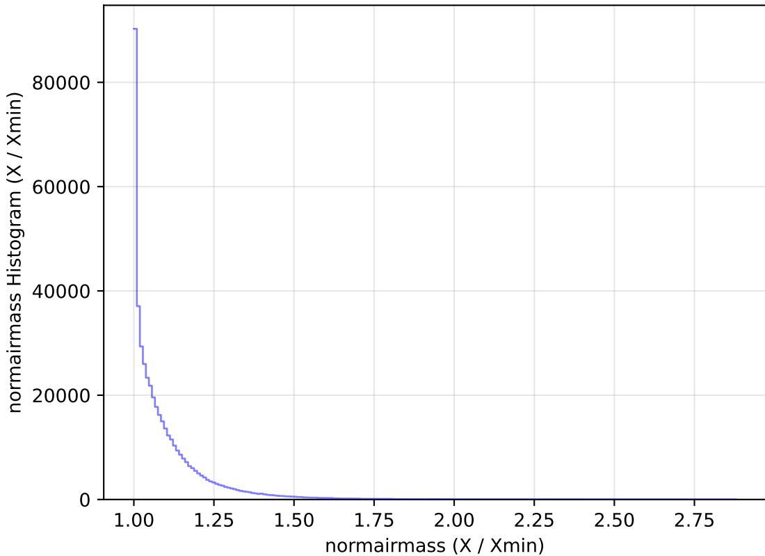
baseline_v2.1_10yrs WFD r band: normairmass Histogram
