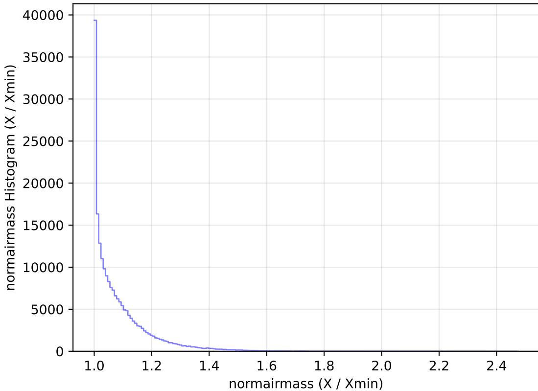
baseline_v2.1_10yrs WFD g band: normairmass Histogram
